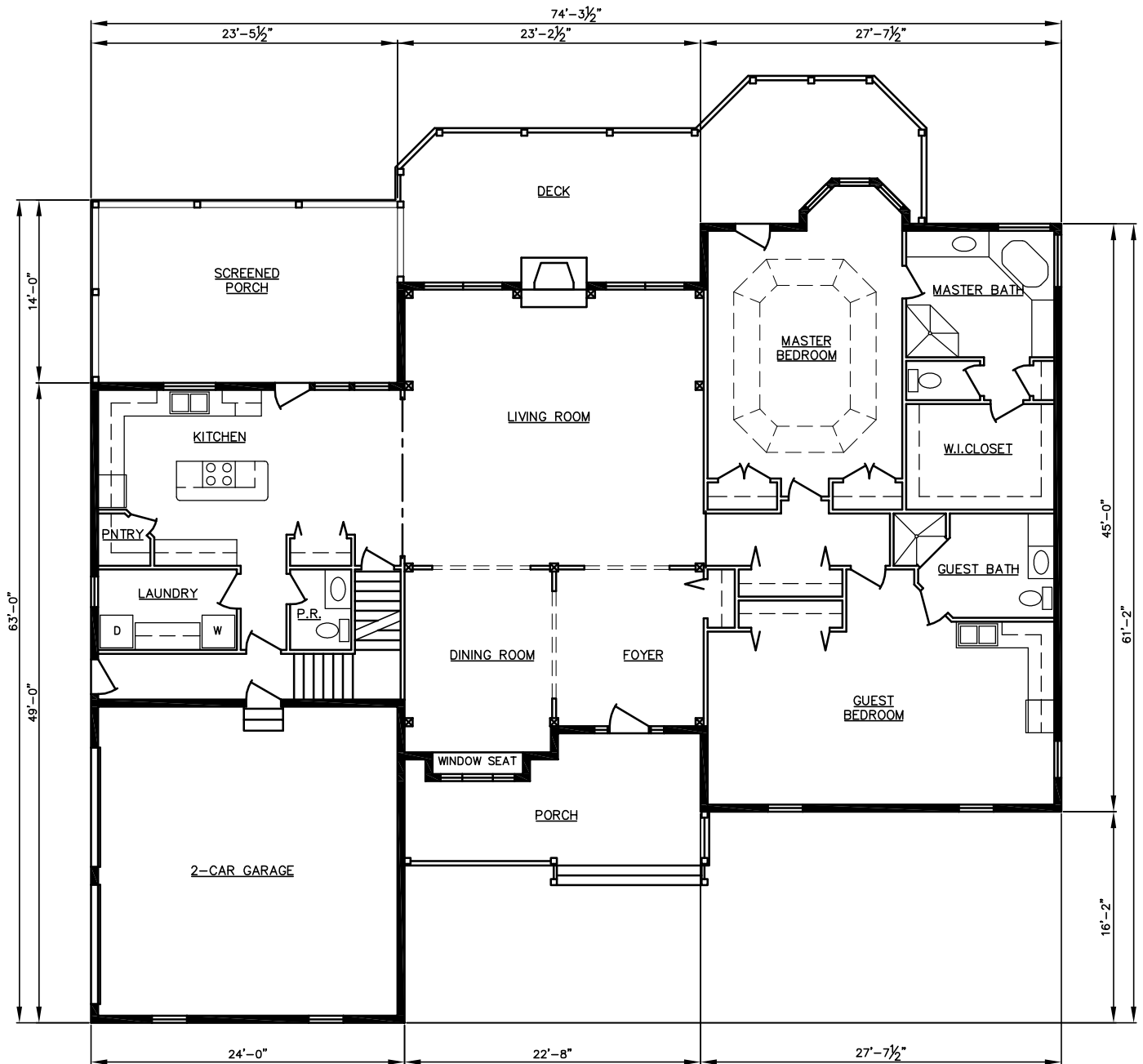
FLOOR PLAN
